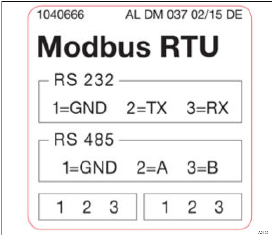
Fig. 1: Modbus Connection Terminals
